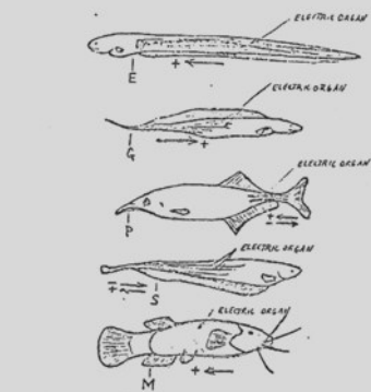
Fig. 1. Principal representatives of fresh-water electric fishes. Arrow indicates direction of current in the electric organs. E = Electrophorus electricus (electric eel) G = Gymnarchus niloticus P = Elephantopus petersii (elephant-nose) S = Sternarchus albifrons (black-ghost) M = Malapterurus electricus (electric catfish)
